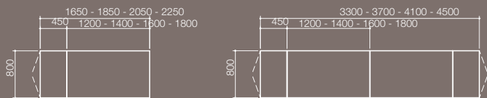
Desks with desk-height storage system Scrivanie con contenitori complanari
