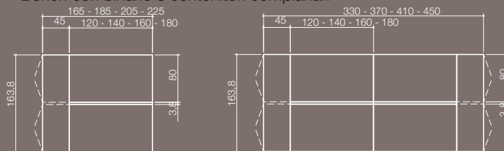
Bench desks with rail and desk-height storage system Bench con binario e contenitori complanari
